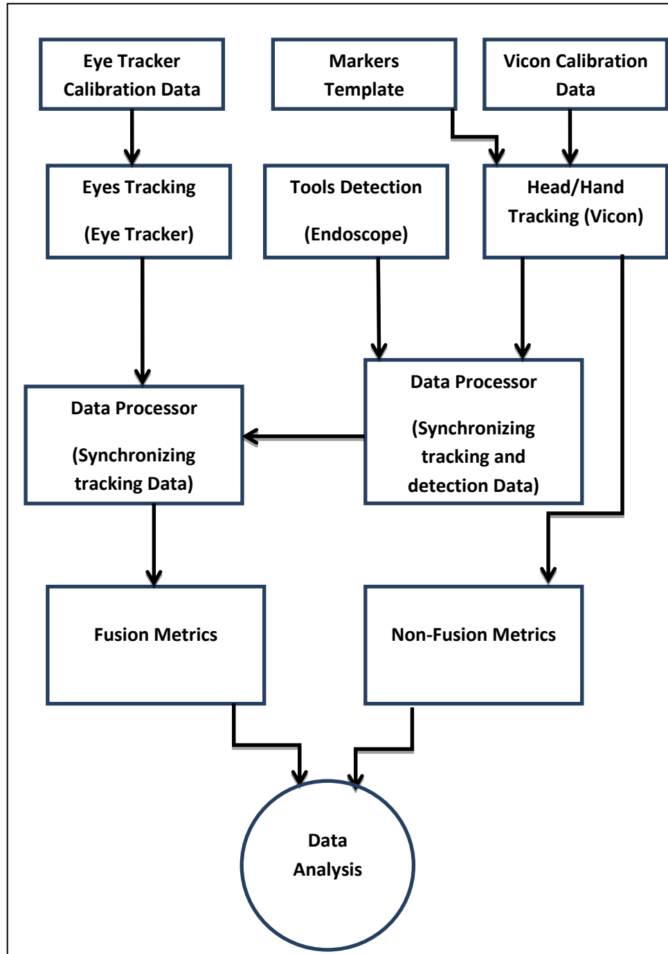
Figure 3.18 Block diagram for tracking hands and head to extract metrics
